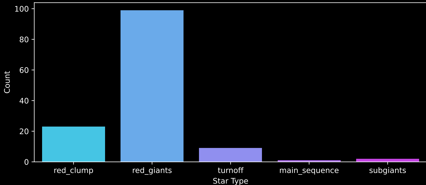
APOGEE DR17 Field: [Sgr_rvvar1] Count plot of Star Type
