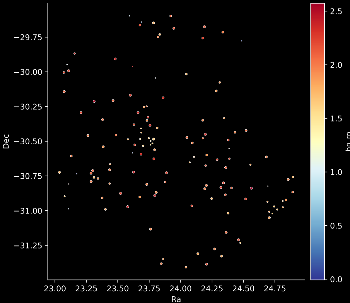
APOGEE DR17 Field: [Sgr_rvvar1] Stars: 134
