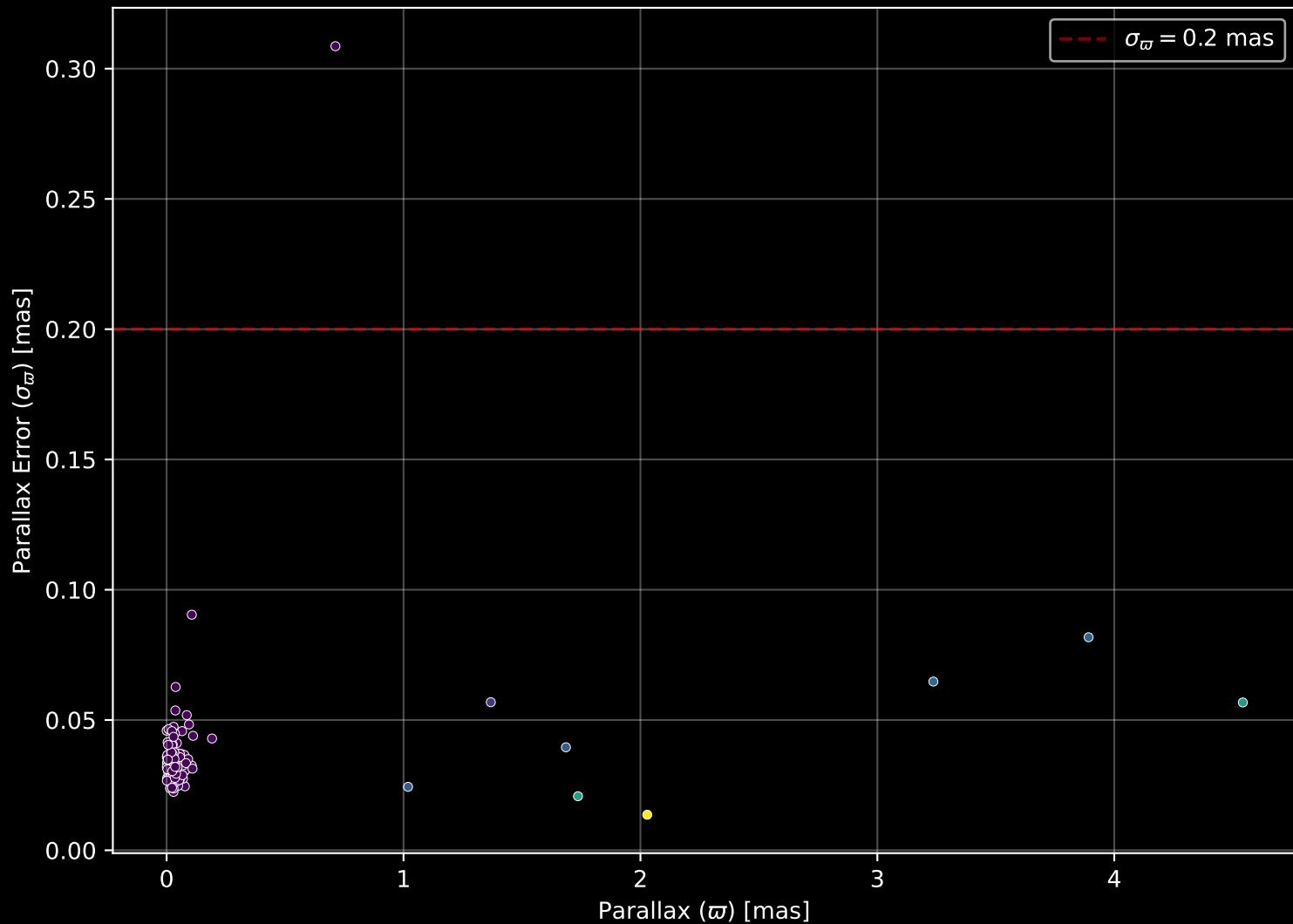
APOGEE DR17 Field: [Sgr_rvvar1] Parallax Quality (n= 134)
