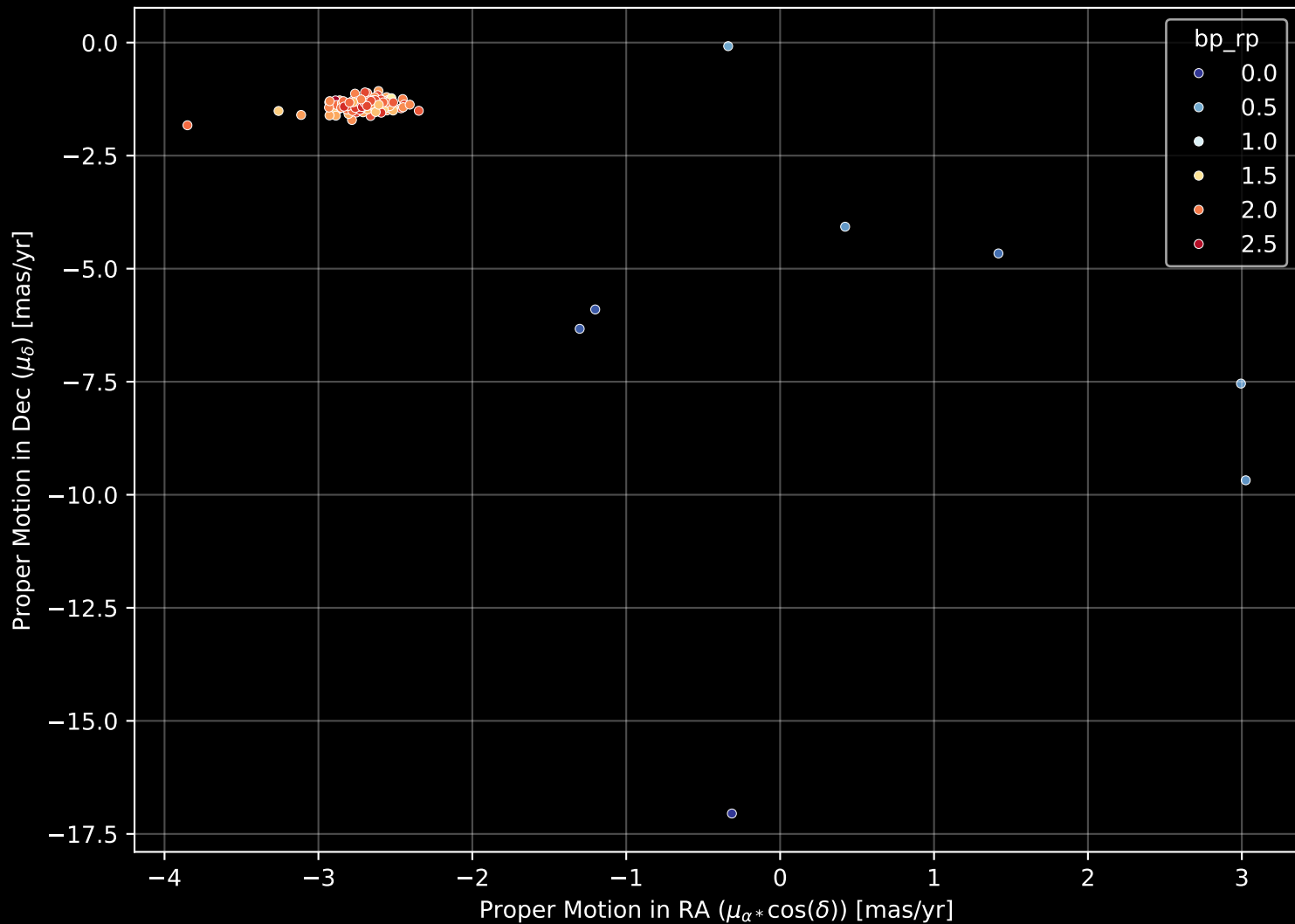
APOGEE DR17 Field: [Sgr_rvvar1] Proper Motion Diagram (n= 134)
