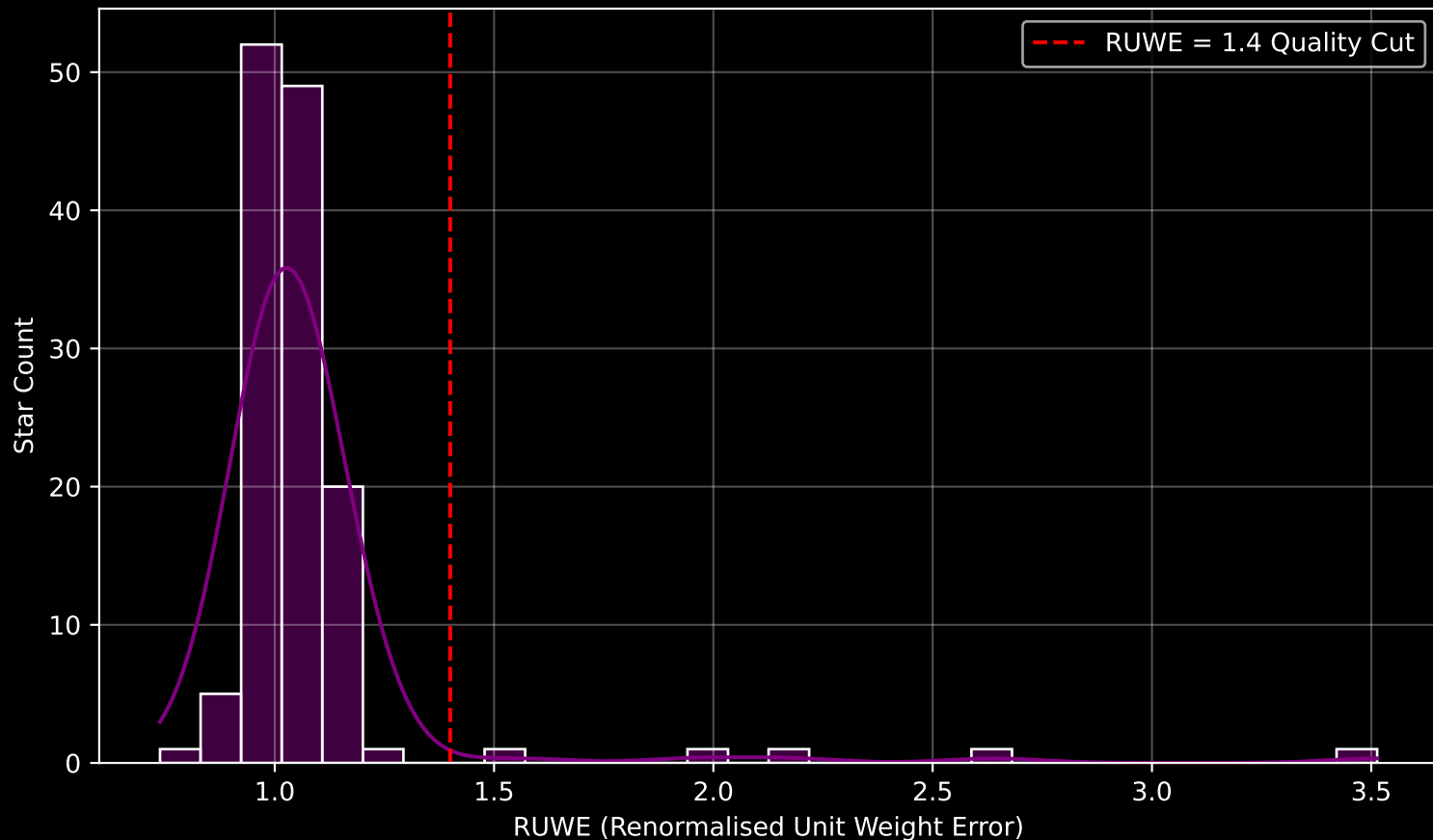
GAPOGEE DR17 Field [Sgr_rvvar1] RUWE Distribution (n= 133)
