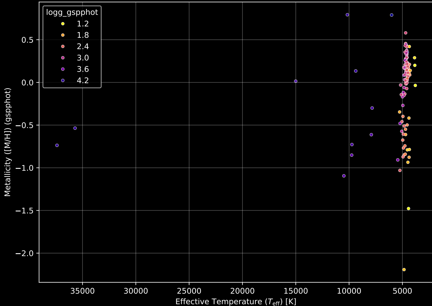
APOGEE DR17 Field: [Sgr_rvvar1] Stellar Population Parameters (n= 134)
