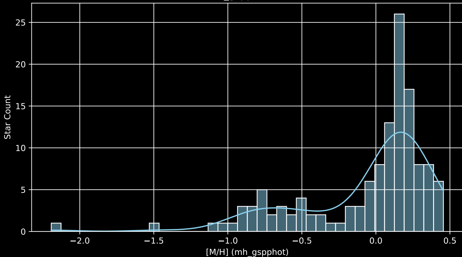
APOGEE DR17 Field: [Sgr_rvvar1 [M/H] (mh_gspphot) (n= 131)
